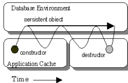
Fig. 4.8: Persistent object.
