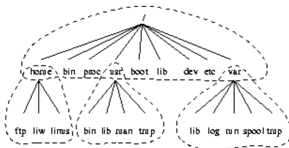
Figure 4-1. Parts of a Unix directory tree. Dashed lines indicate partition limits.
