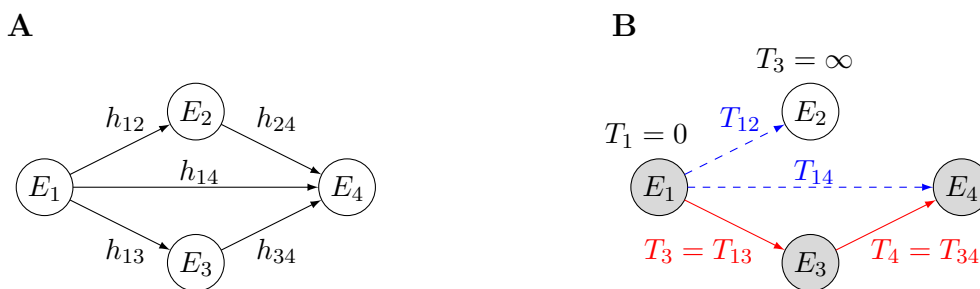
Figure 1: Sample DAG of states and transitions. Panel A shows the states and transition hazards. Panel B shows the potential transition times T_{ij} and the transition times T_j of a simulation where T_{13} < T_{12} . The red solid lines depict the path taken in this particular simulation and the gray circles represent the states visited by the individual. The blue dashed lines represent the potential transitions that never occurred.
