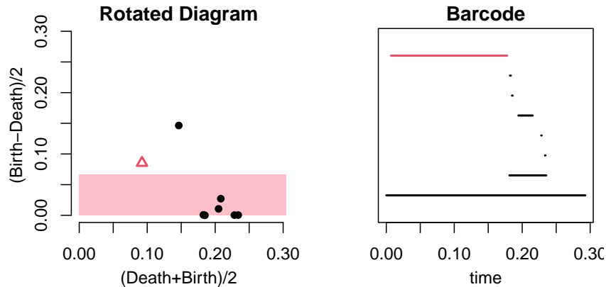
Figure 4: Rotated Persistence Diagram and Barcode
