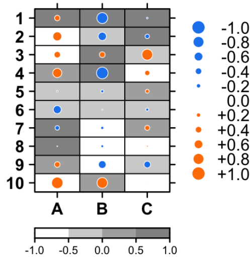
Figure 37: Dotmap with background
