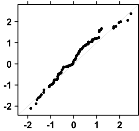
Figure 45: Simple QQ plot comparison
