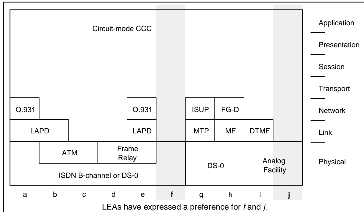
Figure 24: Possible Circuit-Mode CCC Protocol Stacks
