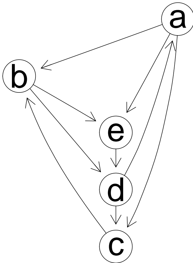
Figure 6: Example Johnson-all-pairs-shortest-paths example
