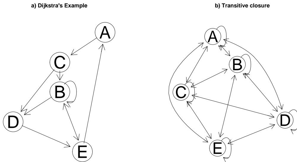
Figure 12: a) The graph for Dijkstra's example. b) The transitive closure of the graph in panel a)
