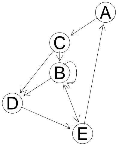
c) Coex2 Example
