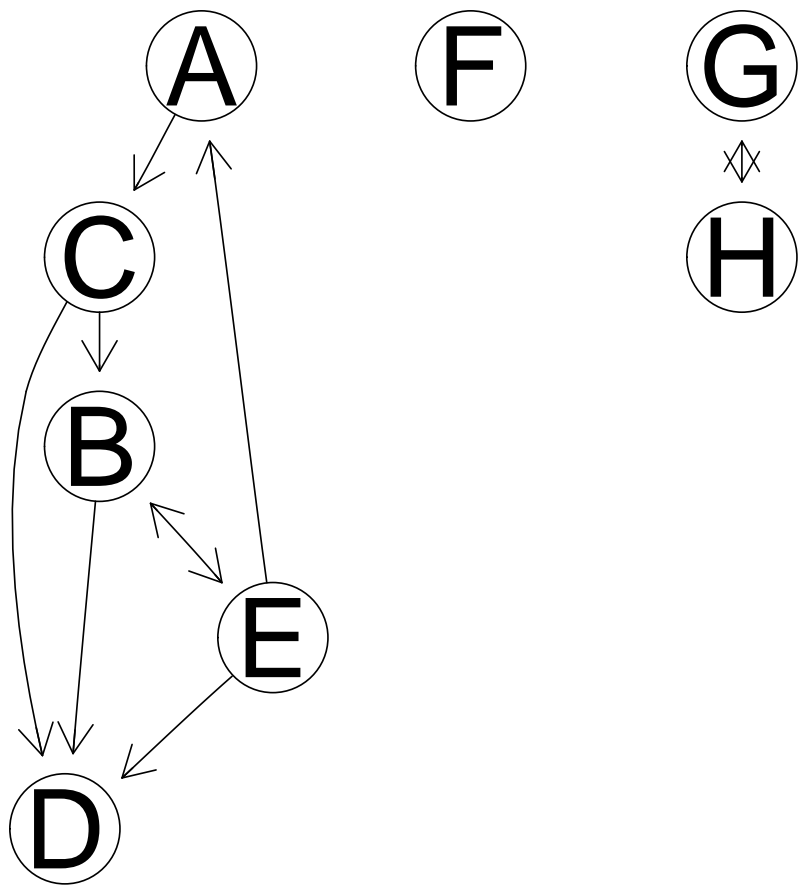
Figure 7: Modified Kruskal MST example from Boost library.
