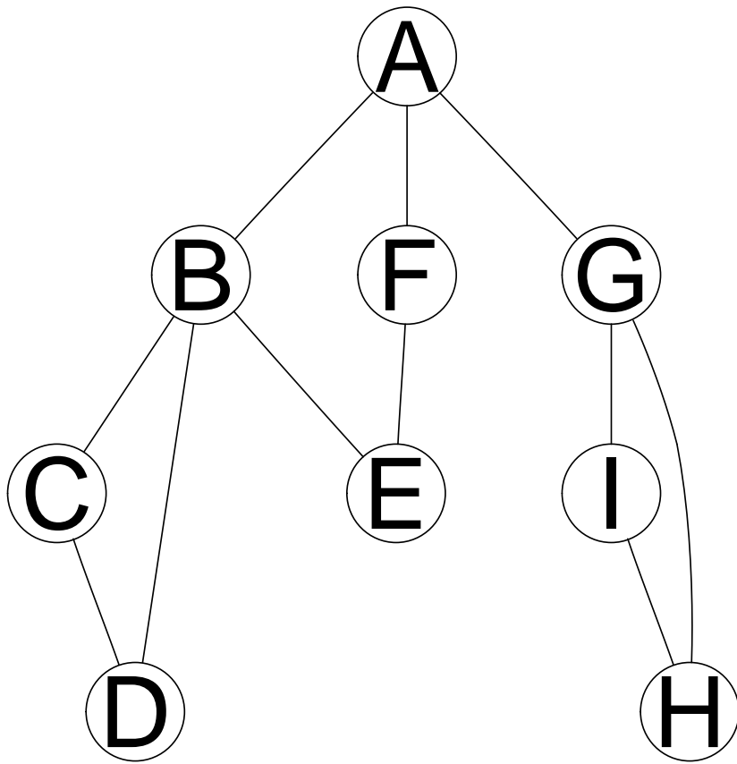
Figure 8: Biconnected components example from Boost library.
