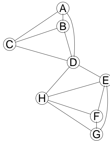
d) HCS Example
