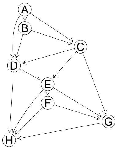
d) Kruskal MST Example
