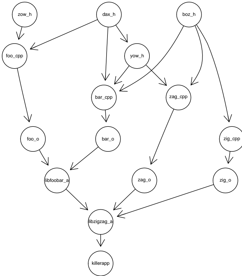
Figure 2: File dependency digraph example from Boost library.
