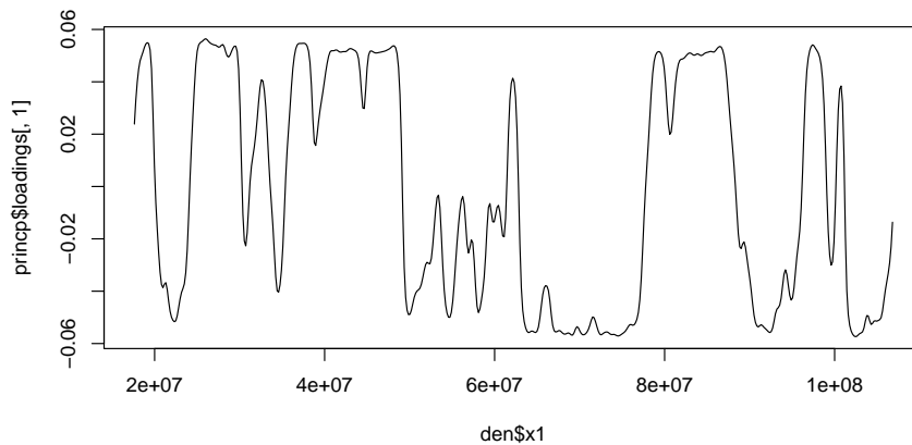
Figure 7: princp$loadings[,1] .
