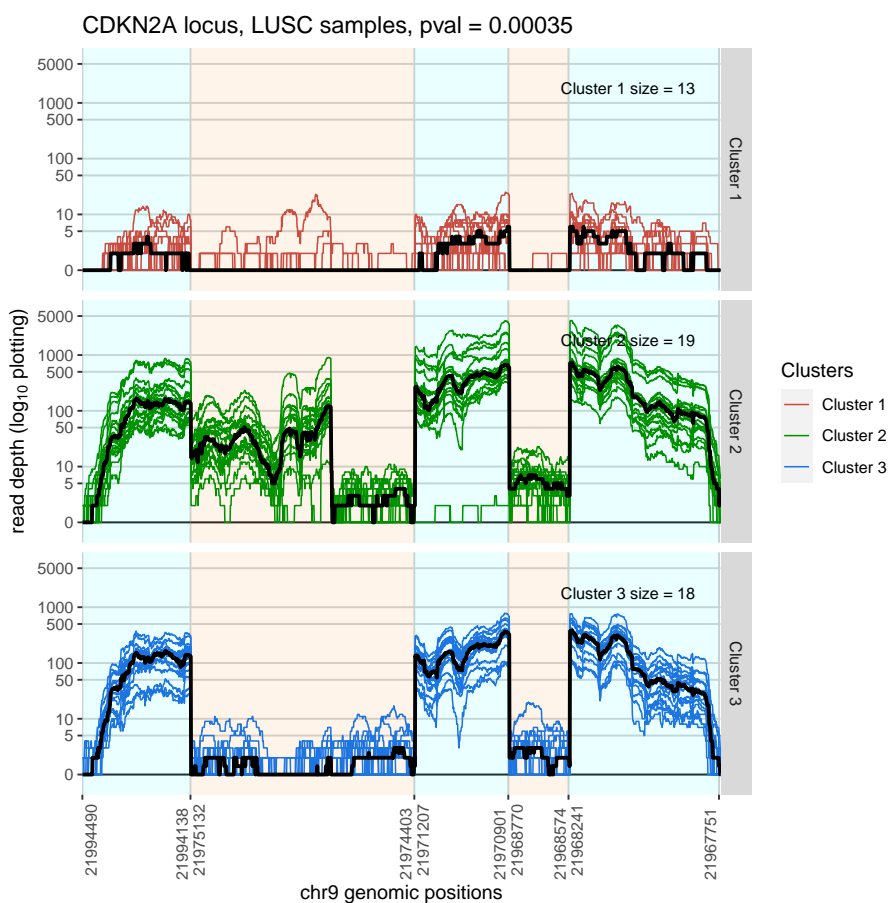
Figure 3: Graphical output from SFigure for lplots = 3
