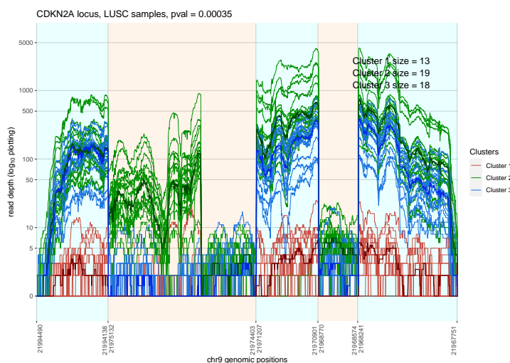
Figure 2: Graphical output from SFigure for lplots = 2 The curves are colored according to class label. The red curves represent a low expression class. There is a large difference in expression of the second exon between the blue and green curves. This difference is reflected in the highly significant p -value.
