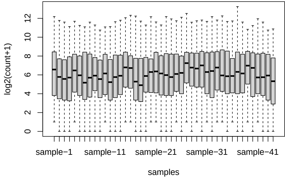
Iteration 2
