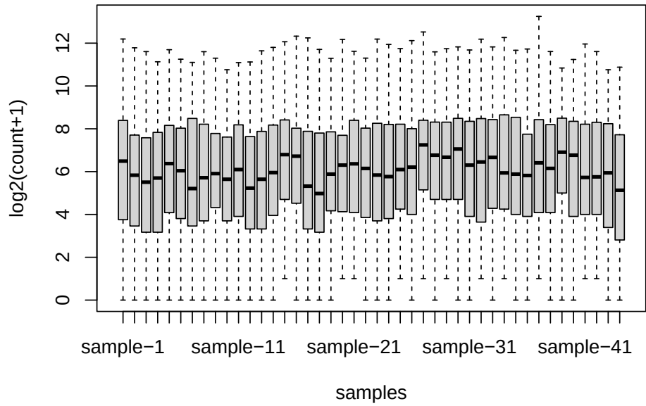
Iteration 4
