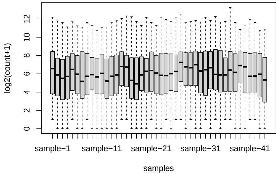
Iteration 4
