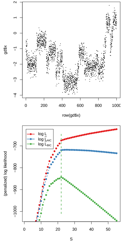
Figure 2: a) simulated data example with nrSeg=22 segments and vertical lines representing the fitted model with S = 22 , selected by maximum \log L_{BIC} . b) log-likelihood \log L , penalized likelihoods \log \tilde{L}_{AIC} and \log \tilde{L}_{BIC} .
