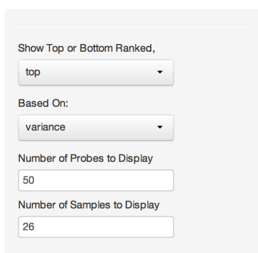
Figure 16: Subset UI
