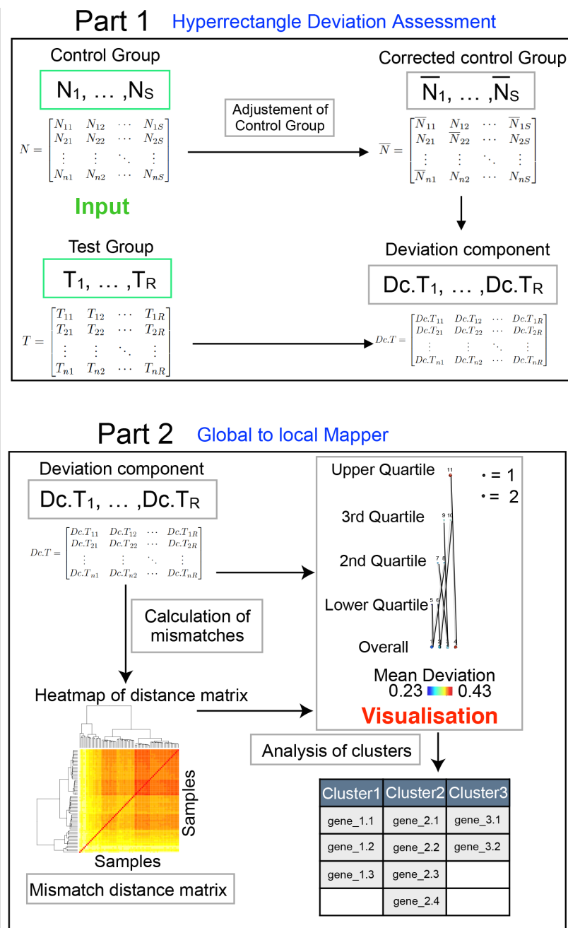
Figure 1: Schematic overview of TTMMap. The inputs (green) are given by two gene expression matrices, the control (N) and the test group (T), rows represent genes and columns samples. In Part 1, TTMMap adjusts the control group for outlier values ( \bar{N}_* ), feature by feature. It calculates deviation from this corrected control group for individual samples in the test group ( Dc.T_* ). In Part 2, TTMMap computes a similarity measure, the mismatch distance (represented as a heatmap) using the deviation components. The Mapper [?] algorithm is used with a two-tier cover to generate a visual representation of the clustering creating a network of global clusters (Overall) and local clusters (1st, 2nd, 3rd, 4th quartile of a filter function). It takes as inputs the mismatch distance and the deviation components.
