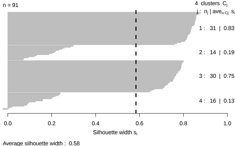
Silhouette plot for K=4 clusters
