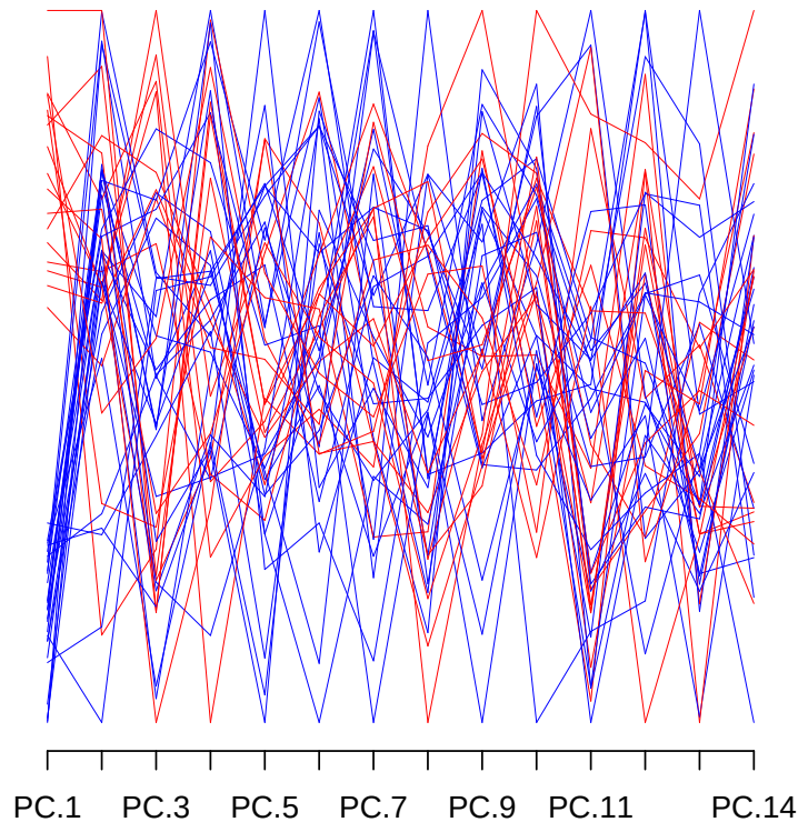
Parallel Coordinates Plot CEU: blue, YRI: red
