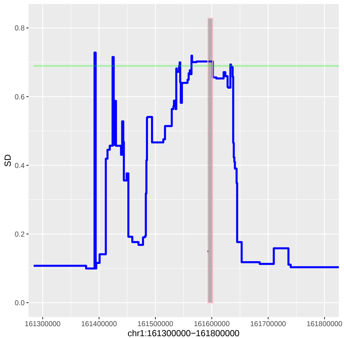
Figure 8: CN polymorphic region at FCGR3 locus, represented by quantiles of the distribution of segregation scores across samples.
